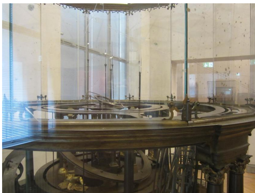
Figure 25.7: The upper level of Neßtfell's machine, which all the planets moving in a tilted plane. (photograph by the author)
